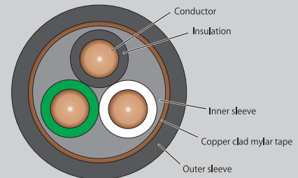
7N-P4040F Cable structure
