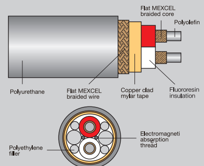
7N-A2500II MEXCEL (Balanced twin-core+shield)
